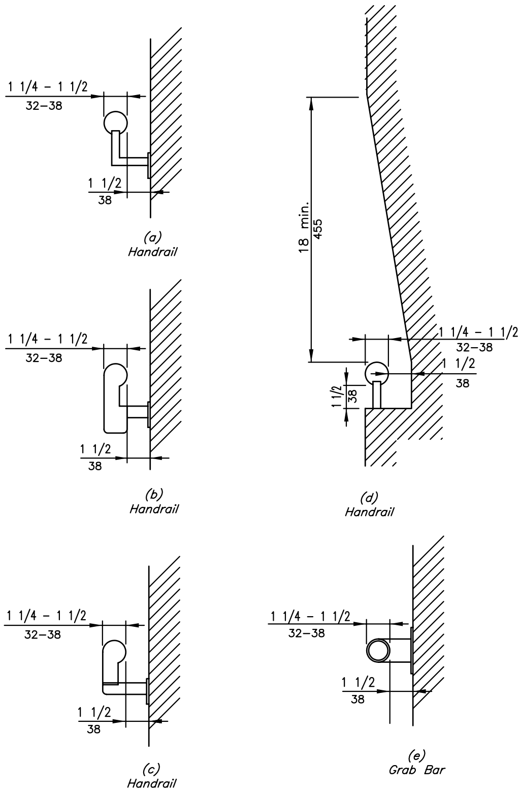
Fig. 39 Size and Spacing of Handrails and Grab Bars
